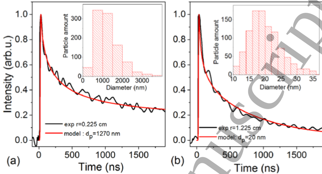
Fig. 7. Measured and fitted LII signals at r=2.25 mm (a) and r=12.25 mm (b) (from ref. [16]).
