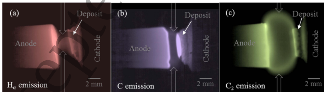
Fig. 4. FFI images of \text{H}_\alpha (a), C I (b), and \text{C}_2 (c) line brightnesses with the arc operated in the low-ablation mode (from ref. [11]).
