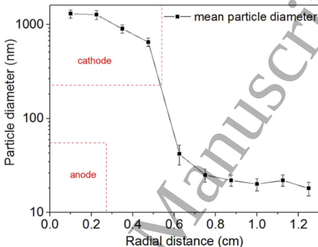
Fig. 8. Mean particle diameter obtained by fitting LII measurements as a function of radial distance from the arc axis (from ref. [16]).
