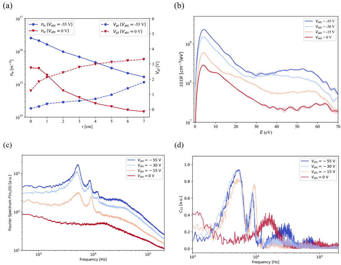
FIG. 2. (a) Radial profiles of electron density n_e and plasma potential V_{pl} , for anticathode bias voltage V_{atc} = -55 V and V_{atc} = 0 V. (b) EEDFs determined by LP at r = 0 cm for varying anticathode bias voltage V_{atc} , with shaded region indicating the standard deviation of the measured EEDF. (c) Fourier spectra of ion density temporal trace determined by IP for varying values of the anticathode bias voltage V_{atc} ; measurements performed at r = 2.3 cm. (d) Cross coherence for varying anticathode bias voltage V_{atc} ; measurements performed at r = 2.3 cm. Parameters are B = 100 G, V_c = 55 V, and p = 0.1 mTorr.
